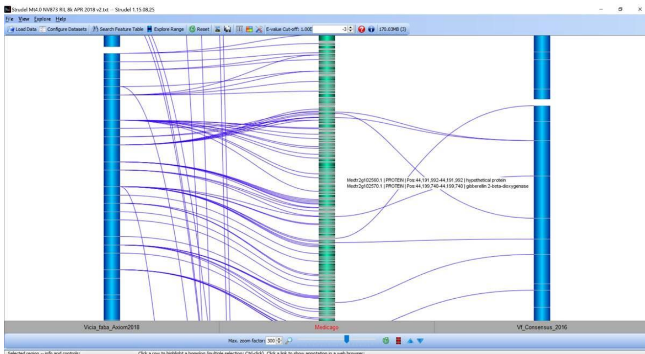
Comparative plot of re-arrangement between Vicia faba old (Vf_Consensus_2016, on the right) and new high resolution consensus genetic map (Vicia faba_Axiom2018, on the left) and Medicago truncatula (in the middle), showing the increase in marker density represented by the new array. (provided by Deepti Agra)
